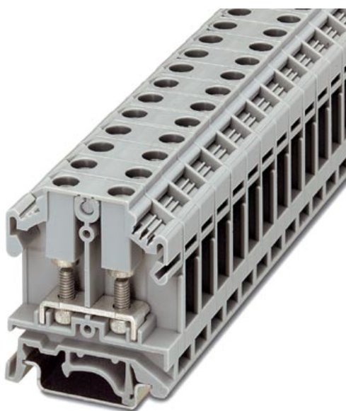
Universal terminal block with bolt connection, cross section: 0.1 - 6 mm 2 , width: 11 mm, color: gray
