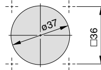
Panel mounting hole
