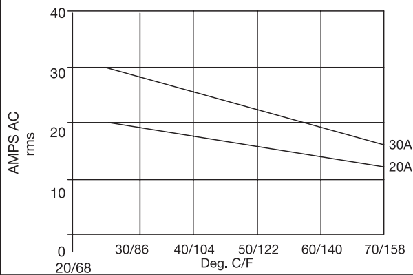
Derating Curve SS20/SS30
