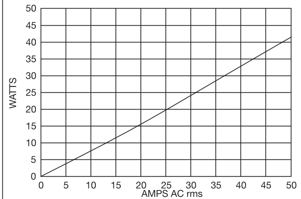
Power Dissipation VS. Load Current SS50
