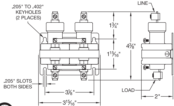
TWO POLE—NORMALLY OPEN
