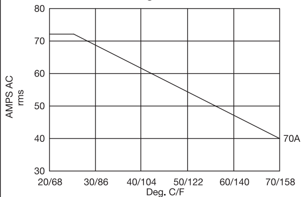
Derating Curve SS70
