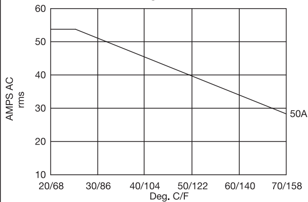
Derating Curve SS50
