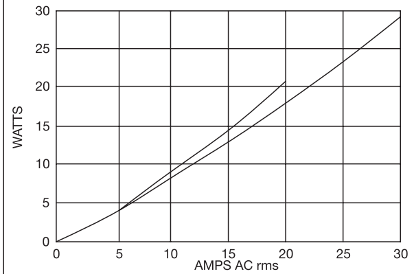
Power Dissipation VS. Load Current SS20/SS30
