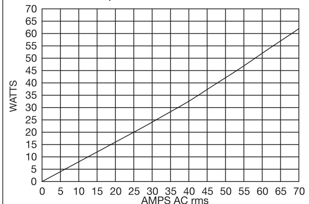
Power Dissipation VS. Load Current SS70
