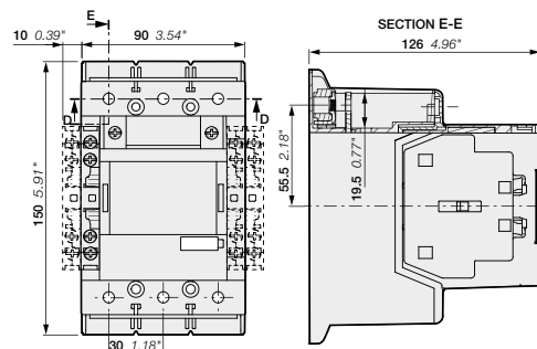
AF116, AF140, AF146-30-11B
