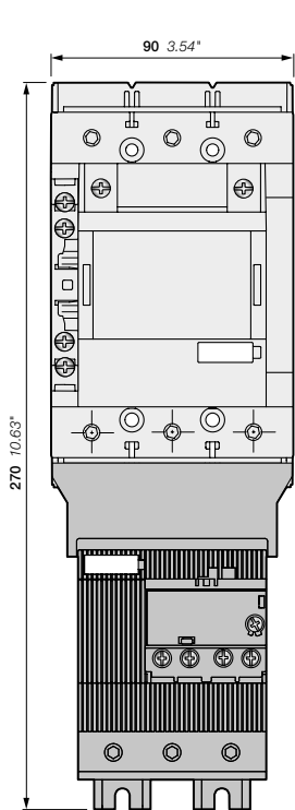
AF116, AF140, AF146-30-11(B) + EF146 electronic overload relay
