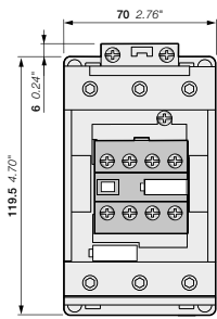
AF80, AF96 + CA4 4-pole auxiliary contact block
