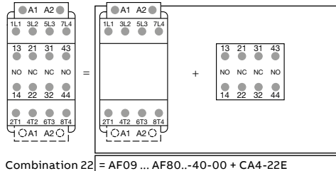
Combination 22 = AF09 ... AF80...-40-00 + CA4-22E
