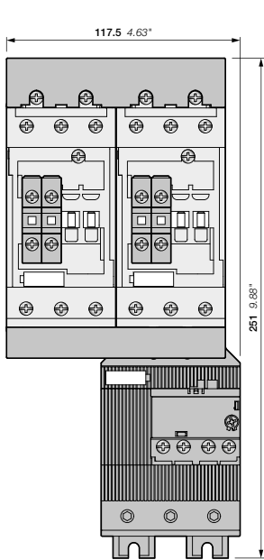
AF40, AF52, AF65 + BER65-4, VM96-4 + EF65 electronic overload relay
