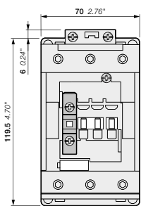
AF80, AF96 + CA4, CC4 1-pole auxiliary contact block
