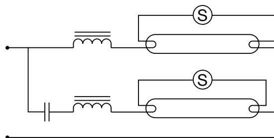
Serial compensation in dual mounting
