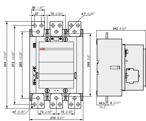
AF1250 Main dimensions mm, inches
