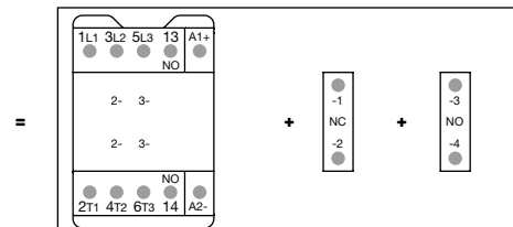
ASL09 ... ASL16-30-10S + CA3-01S + CA3-10S
