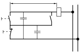
Wiring diagram B Via momentary pushbutton plus hold-in contact and 3-core cable (with a capacity of 2 x 0.2 = 0.4 μF/km, for example).
