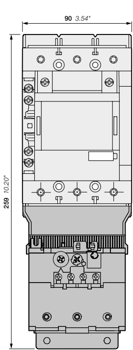
AF116, AF140-30-11(B) + TF140 thermal overload relay
