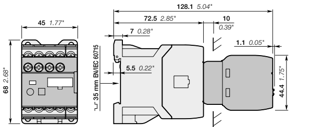
NSL22E, NSL31E, NSL40E + TEF3 electronic timer
