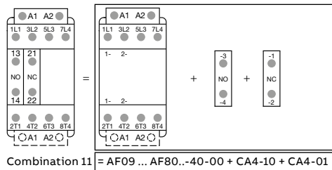
Combination 11 = AF09 ... AF80...-40-00 + CA4-10 + CA4-01
