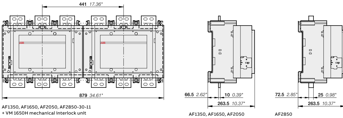
AF1350, AF1650, AF2050
