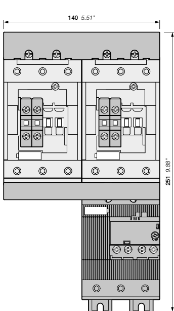
AF80, AF96 + BER96-4, VM96-4 + EF96 electronic overload relay
