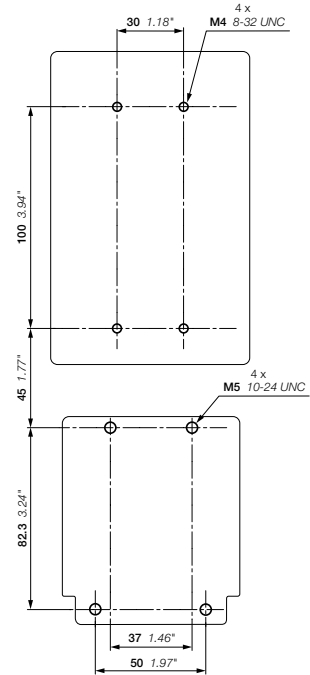
AF116, AF140-30-11(B) + TF140 thermal overload relay
