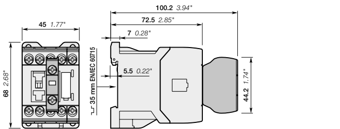
NSL22E, NSL31E, NSL40E + CA3 front-mounted 1-pole auxiliary contact block
