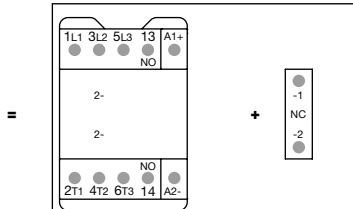
ASL09 ... ASL16-30-10S + CA3-01S
