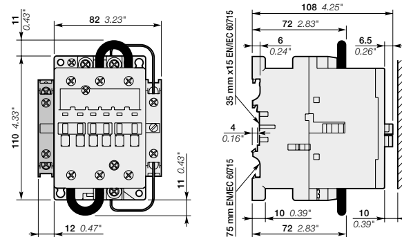
GAE75-10-11 Main dimensions mm, inches
