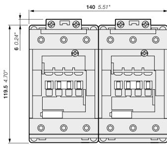
AF80, AF96 + VM96-4 mechanical interlock unit
