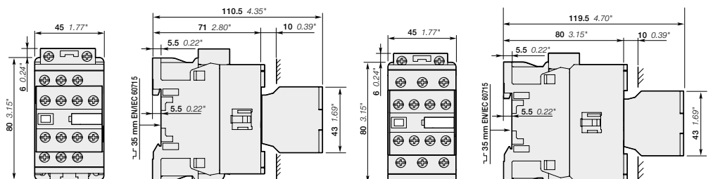
AF09Z, AF12Z, AF16Z Main dimensions mm, inches
