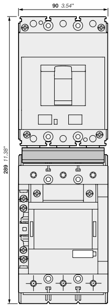
XT2S 160 + Ekip M-LIU In160 + BEA140/XT2 + AF116, AF140, AF146
