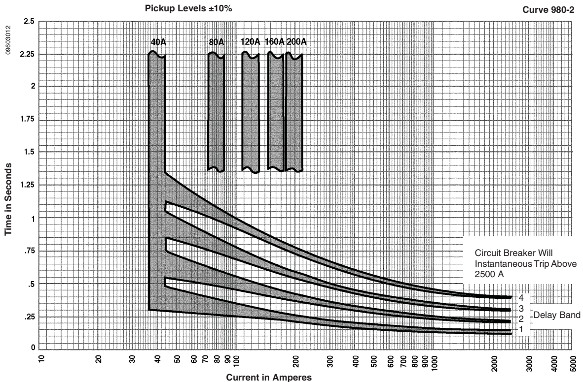
Figure 99: Ground Fault Module GFM250JD Trip Curve
