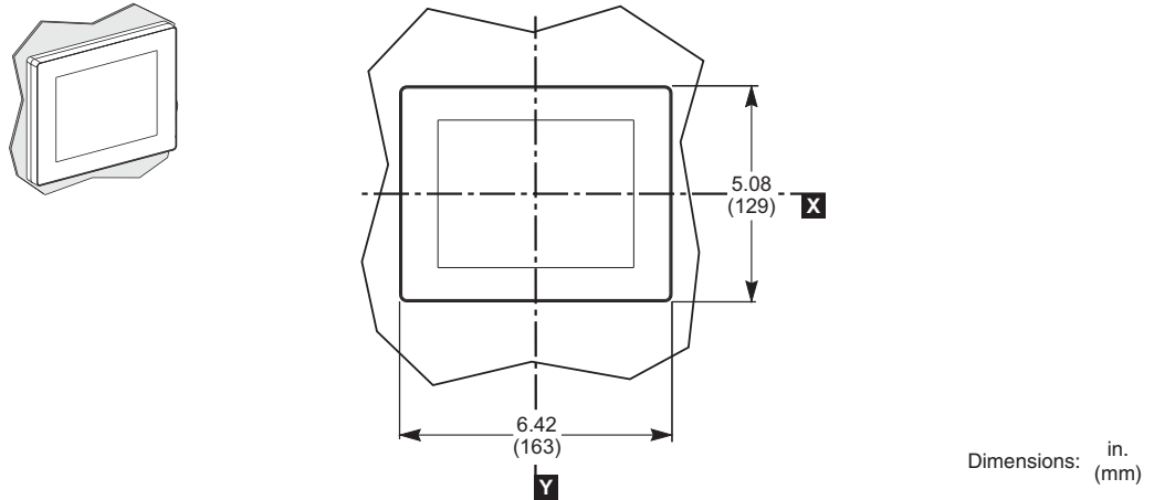
Figure 68: FDM128 Switchboard Display Mounting on Panel
