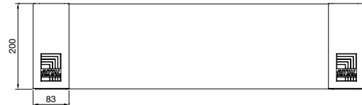
Base/plinth, trim panels, solid, 200 mm (8 in.) high, front view
