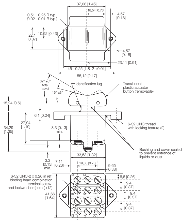
Figure 6. TP Series: Four pole, above panel mounting
