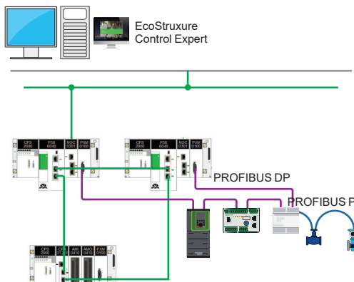
Redundant (HSBY) topology to connect the PROFIBUS DP master X80 module to M580/X80 platforms with PMEPM0100
