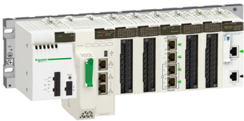
Modicon X80 modules platform with Modicon M580 processor
