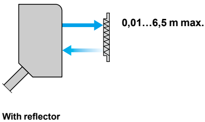
With reflector
