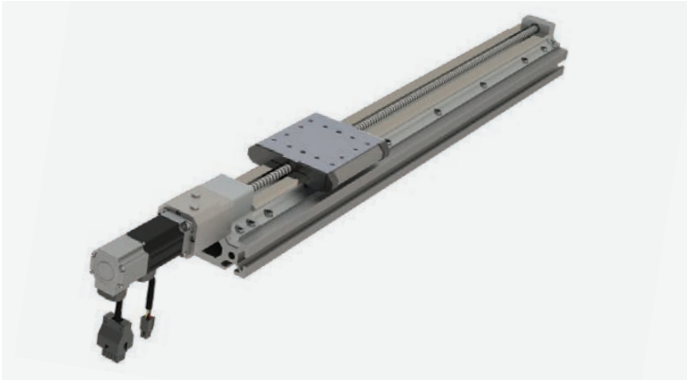
LoPro®: A signature product of BWC, the LoPro® actuator uses the DualVee® wheel and track technology. Available in belt, screw or chain driven options, this is ideal for long applications and harsh environments.
