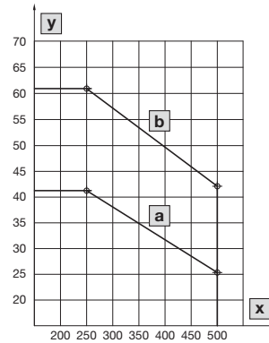
Short-circuit resistance diagram 9340.000/9340.050
